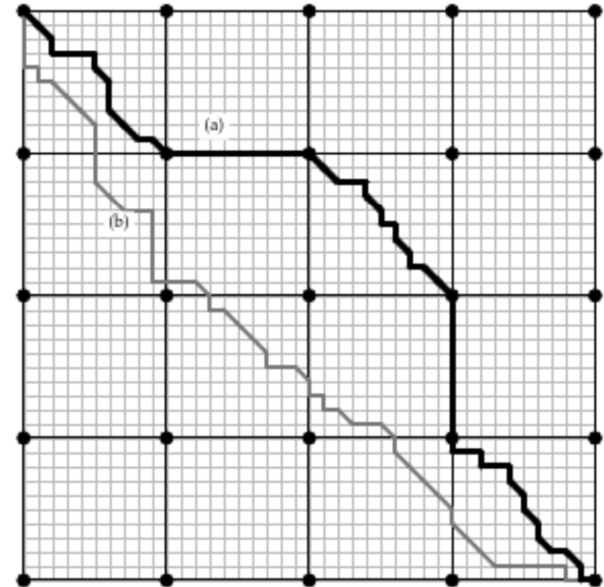
Figure 7.4 Two paths in a 40 \times 40 grid partitioned into 16 subgrids of size 10 \times 10 . The black path (a) is a block path, while the gray path (b) is not.
